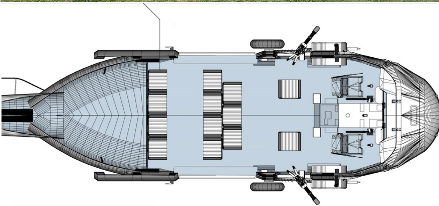
UH-60 top view of the cabin and cockpit
